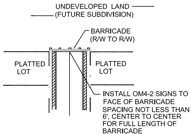
SIMPLE DEAD-END
