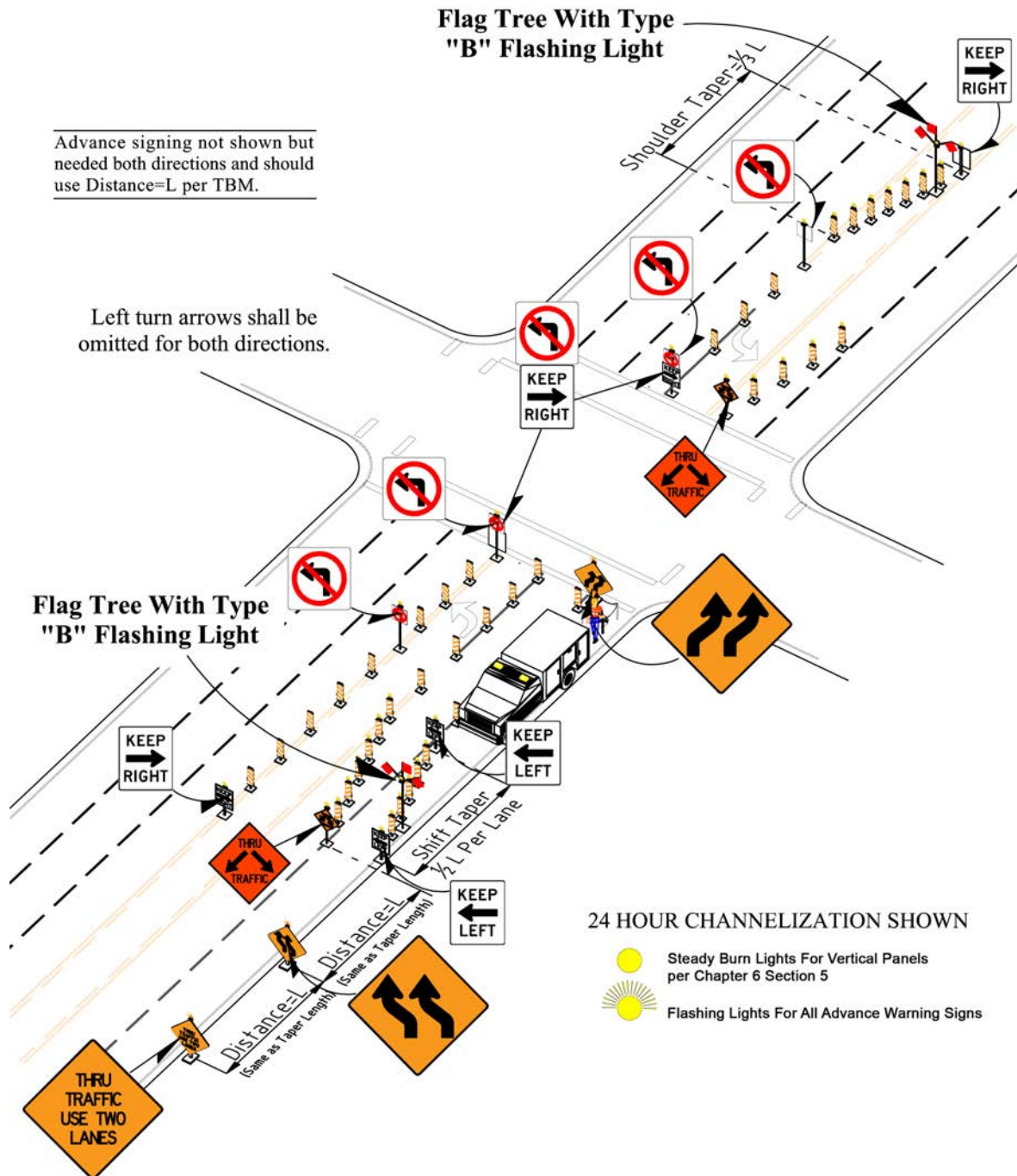
Figure 30 – Nearside Thru/Right Lane Closed (Maintain two thru by prohibiting left turns)
