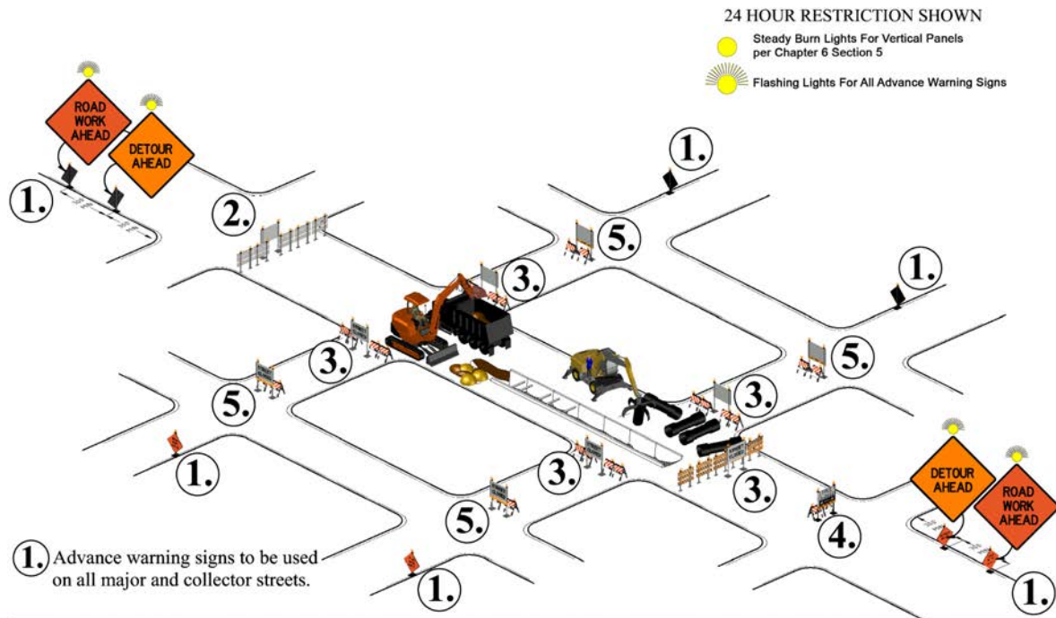
Figure 22 – Street Closure Signing (Hard and Soft)
