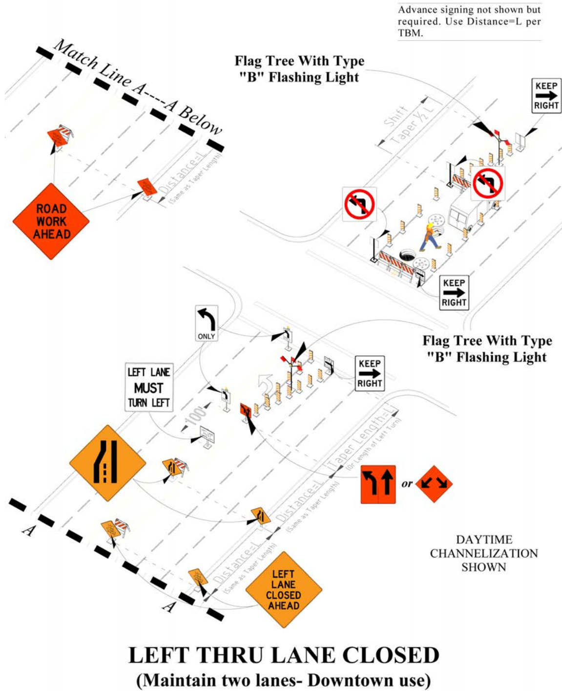
Figure 24 – Thru Lane Closed (Maintain Two Lanes – Downtown use)
