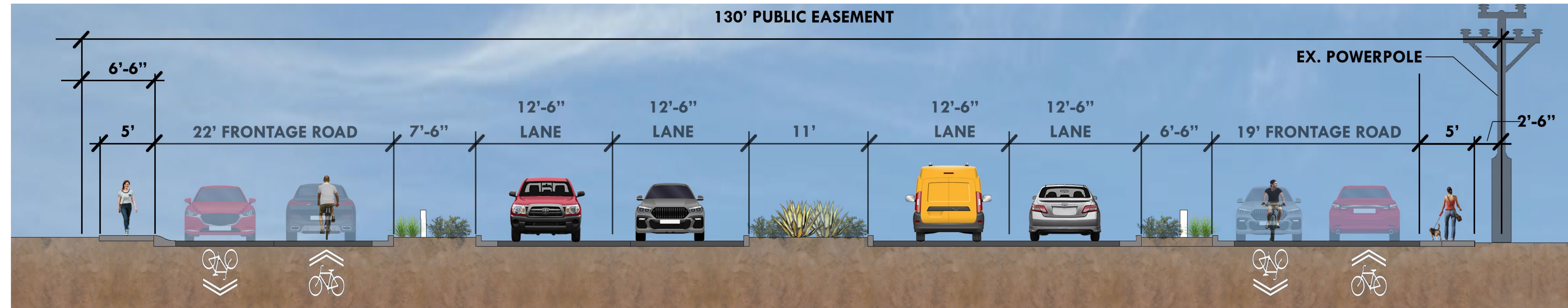
ALTERNATIVE 1 - NEW SIDEWALKS
