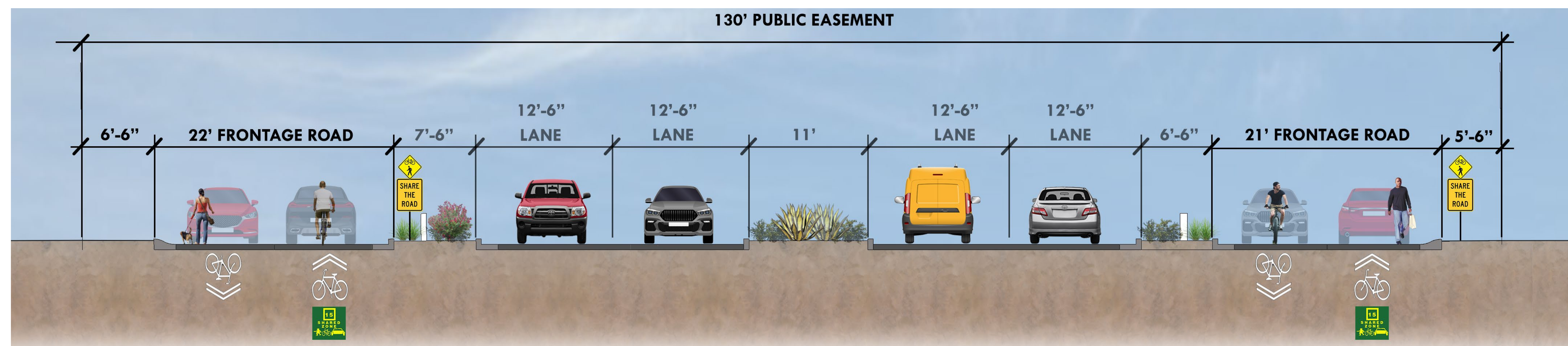
ALTERNATIVE 2 - YIELD STREET WITH INTERSECTION LANDINGS
